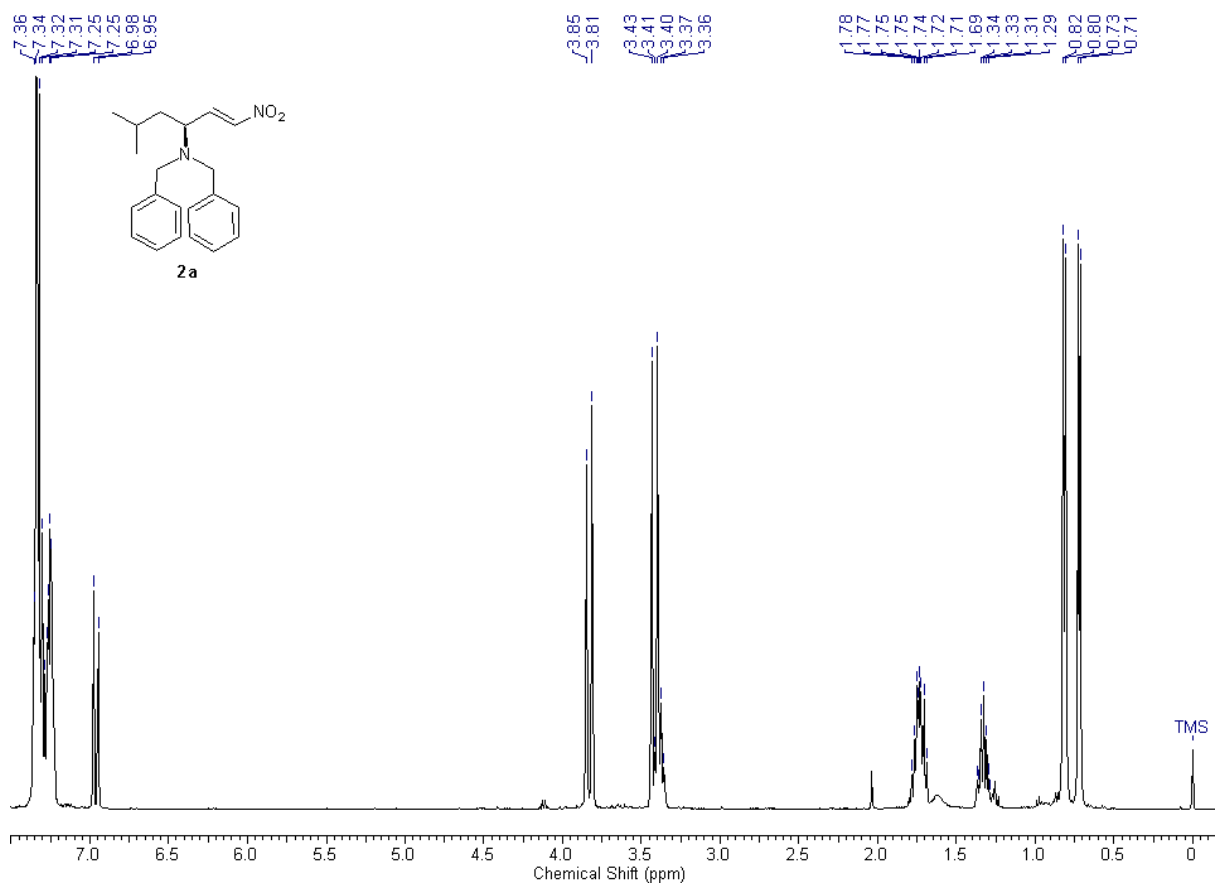
Spectrum 1 - ^1\text{H} NMR of 2a
