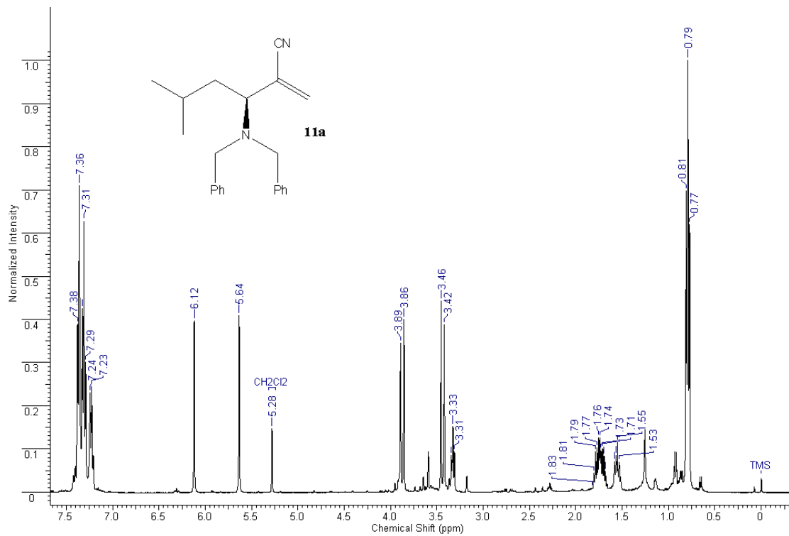
Spectrum 7 - 1 H NMR of 10a
