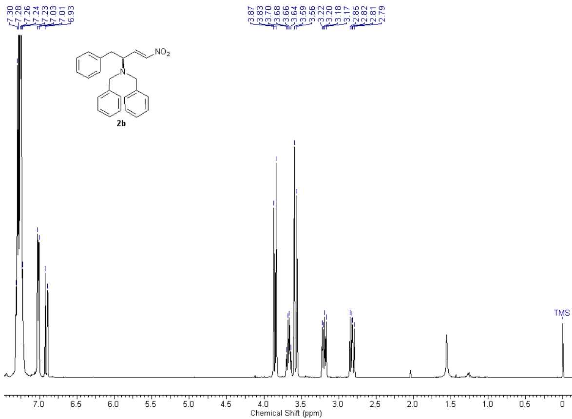
Spectrum 2 - ^1\text{H} NMR of 2b
