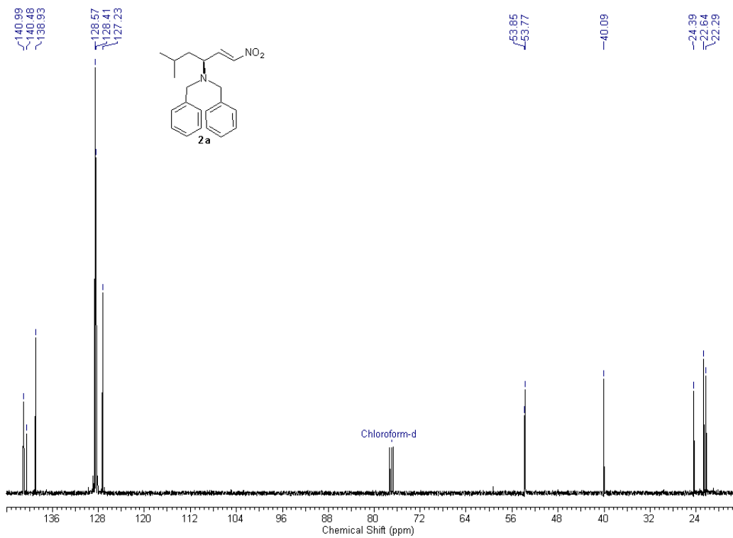
Spectrum 4 - 13 C NMR of 2a
