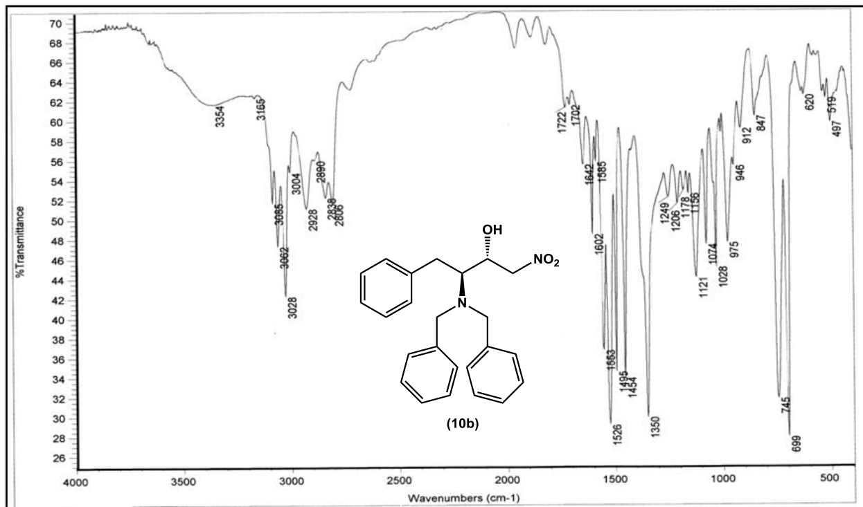
Spectrum 9 – I.R. of 10b
