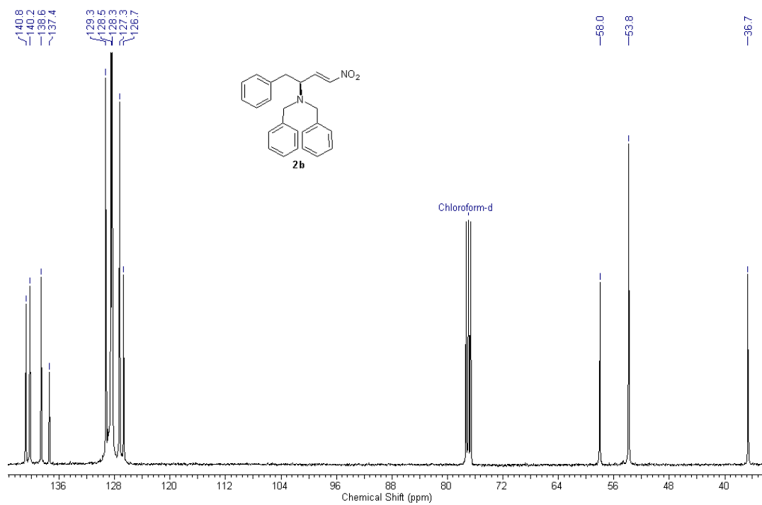
Spectrum 5 – ^{13}\text{C} NMR of 2b
