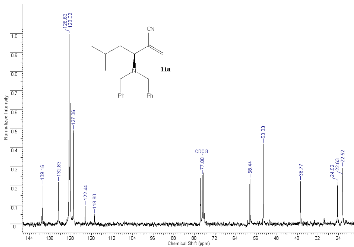
Spectrum 8 - 13 C NMR of 11a
