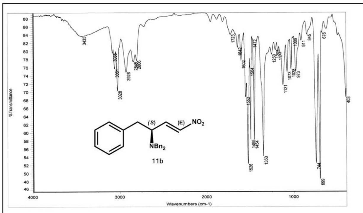
Spectrum 10 – I.R. of 11b
