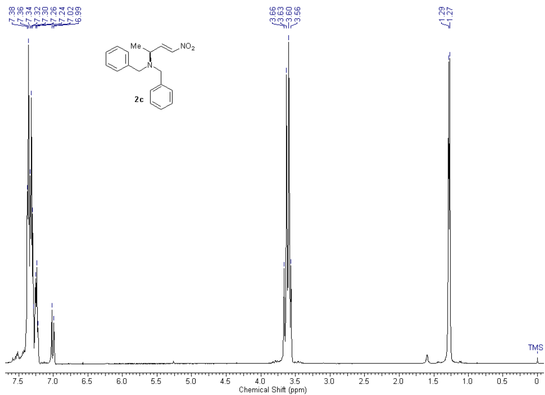
Spectrum 3 - 1 H NMR of 2c
