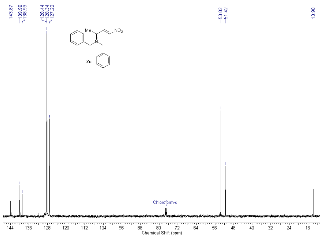
Spectrum 6 - ^{13}\text{C} NMR of 2c
